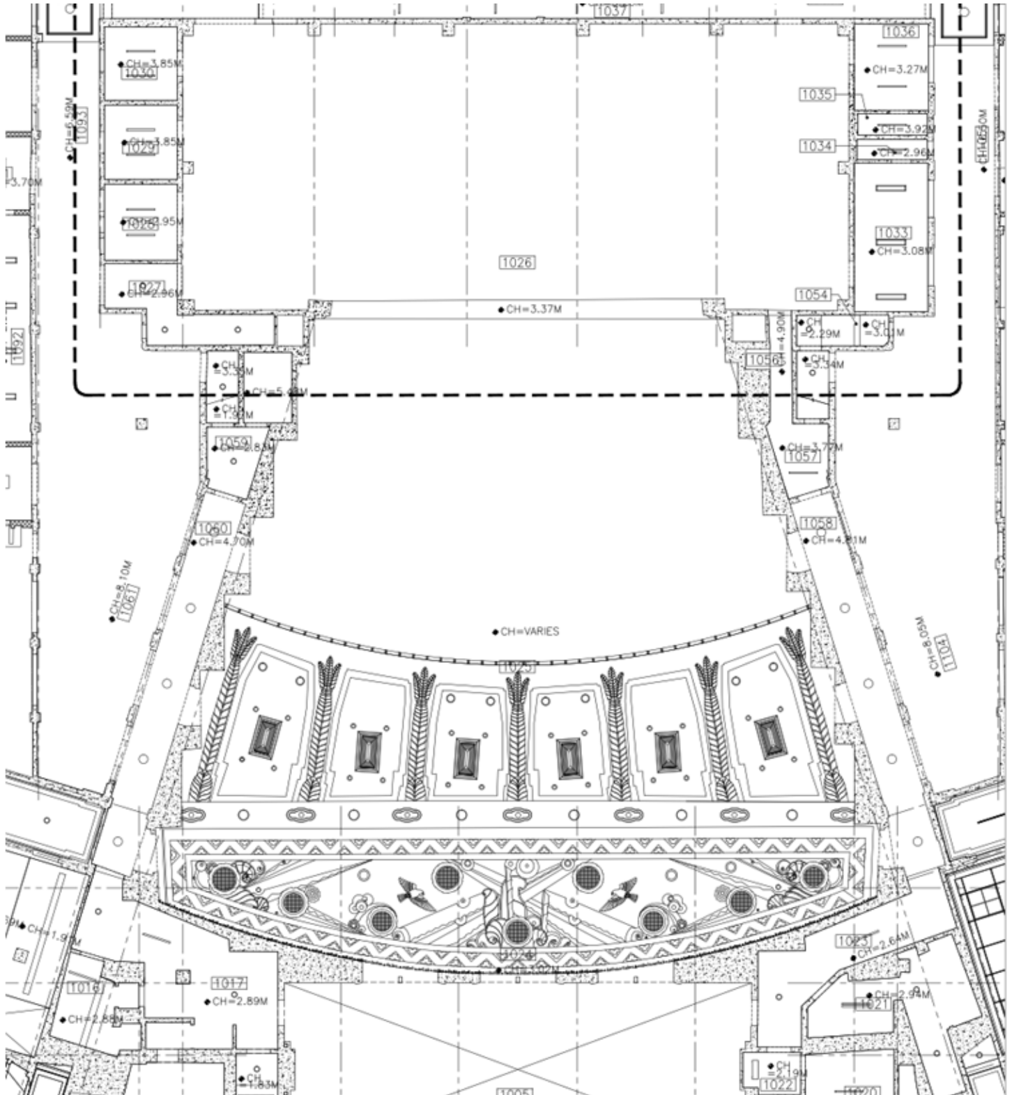
MAIN THEATRE : GROUND FLOOR REFLECTED CEILING PLAN
